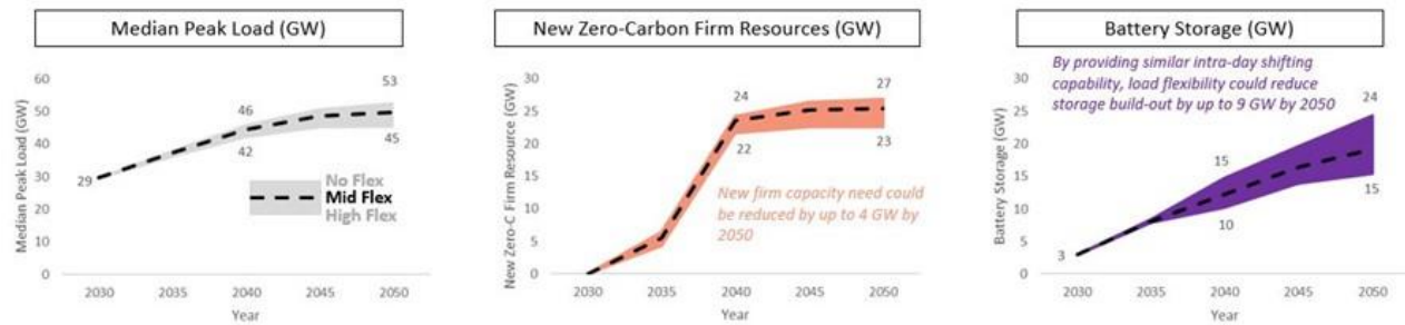
Figure 57. Electric System Resource Mix Impacts of Load Flexibility
