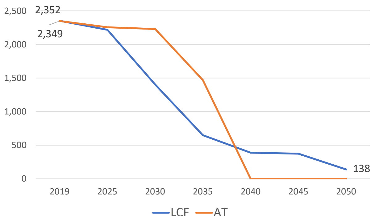
FIGURE 42. OTHER FOSSIL GENERATION: CAPACITY INSTALLED (MW)
