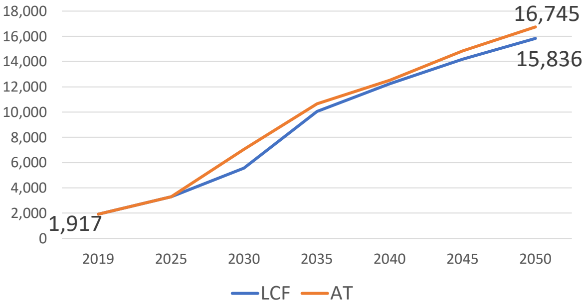
FIGURE 12. ONSHORE WIND: CAPACITY INSTALLED (MW)
